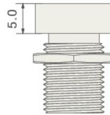
3: High Head
