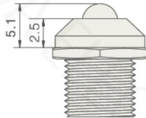
2: Middle Head
