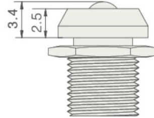
1: Small Flat Head
